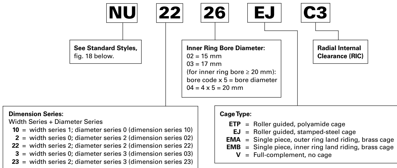
Fig. 17. Metric ISO radial cylindrical roller bearings nomenclature.
