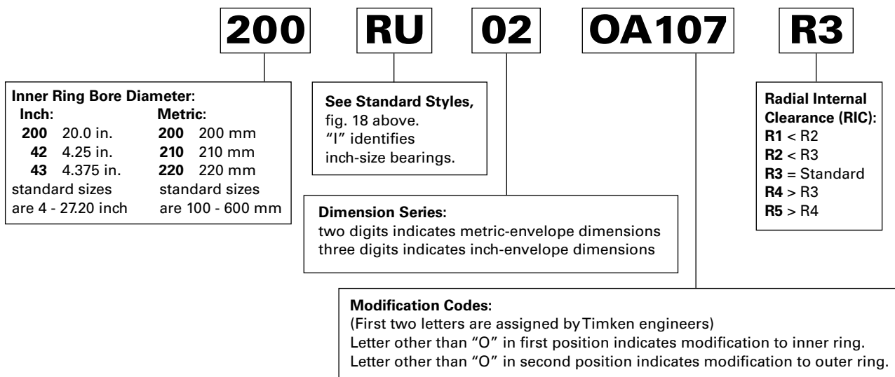
Fig. 19. ABMA radial cylindrical roller bearings nomenclature.
